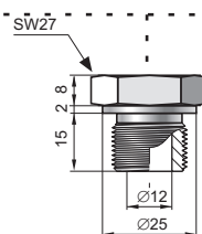
GP type P type G1/2", Ø12 hole M20×1.5, Ø12 hole
